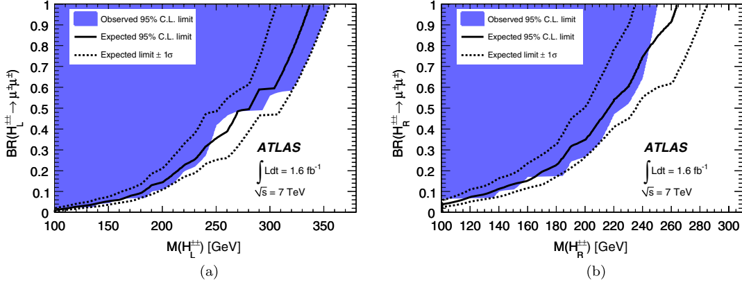
FIG. 3 (color online). Exclusion region at 95% C.L. of the H^{\pm\pm} mass as a function of the branching ratio to muon pairs, BR(H^{\pm\pm} \rightarrow \mu^{\pm}\mu^{\pm}) , for a) H_L^{\pm\pm} bosons and b) H_R^{\pm\pm} bosons. The shaded areas show the observed exclusion region, the solid lines show the expected exclusion region, and the dashed lines show the \pm 1\sigma variations of the expected exclusion region.
