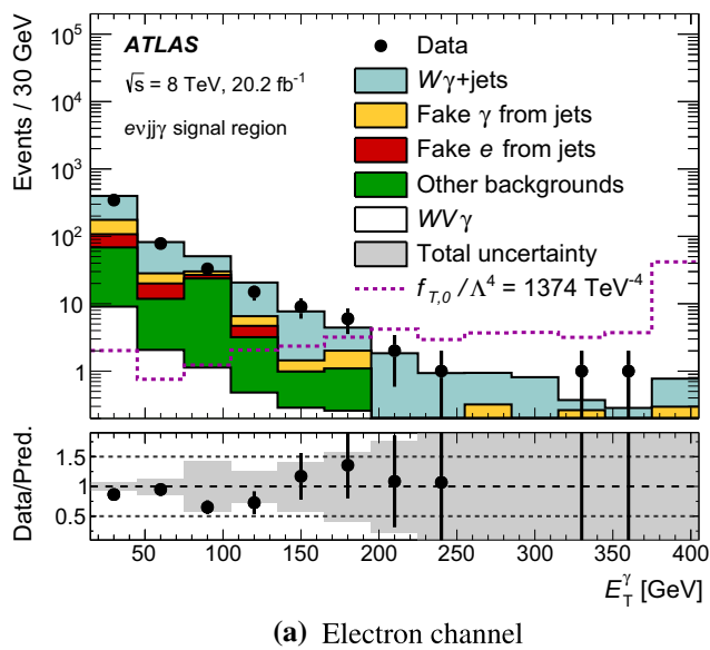
Fig. 5 Observed and expected transverse energy distributions of the photon with the highest E_T in the signal region in the a electron and b muon channels of the semileptonic analysis. The data are shown together with the predicted signal and backgrounds. Also indicated is the expected event yield for a reference model describing aQGCs with
