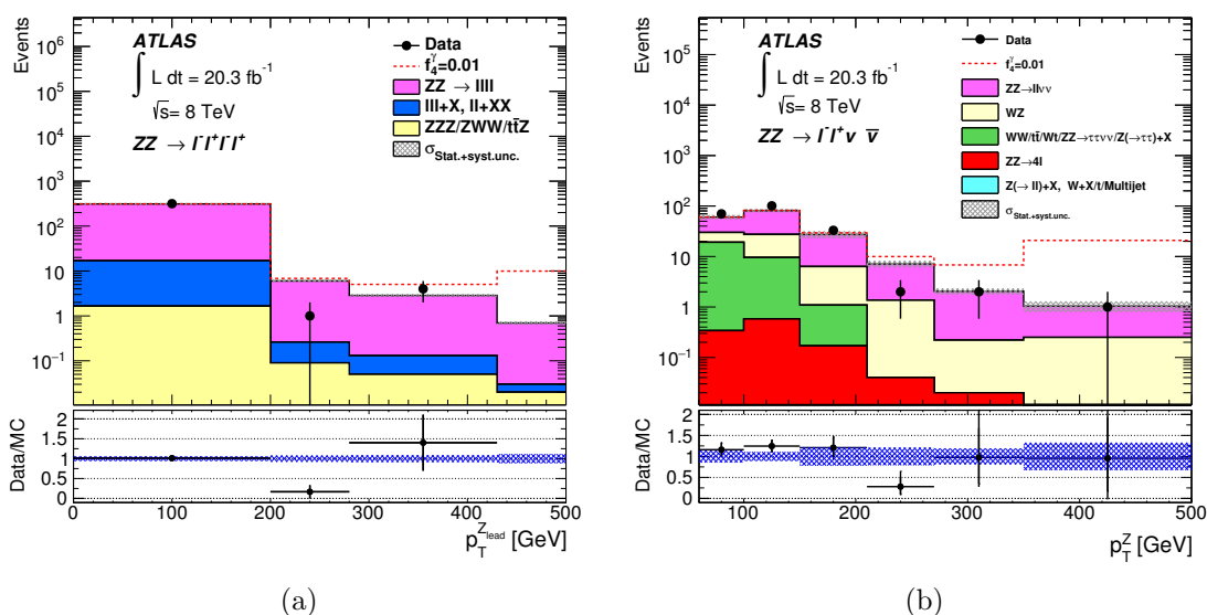
Figure 8. Data and SM prediction of the p_T^Z distribution for the (a) ZZ \rightarrow \ell^- \ell^+ \ell'^- \ell'^+ and (b) ZZ \rightarrow \ell^- \ell^+ \nu \bar{\nu} channels. The expected contribution from the aTGC point with f_4^\gamma = 0.01 is also shown.
