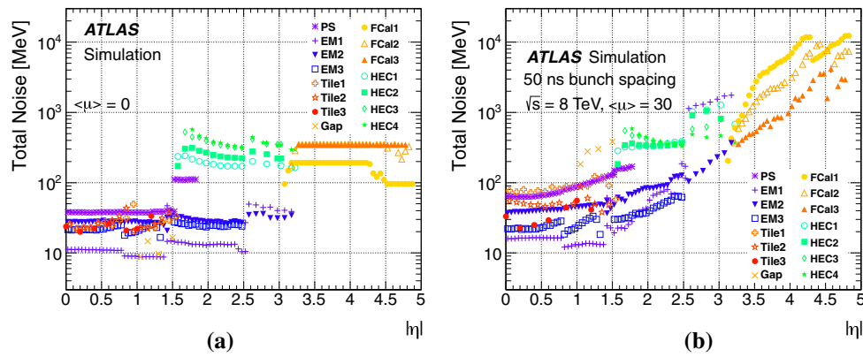
Fig. 2 a Per-cell electronic noise ( \langle \mu \rangle = 0 ) and b total noise per cell at high luminosity corresponding to \langle \mu \rangle = 30 interactions per bunch crossing with a bunch spacing of \Delta t = 50 ns, in MeV, for each calorimeter layer. The different colours indicate the noise in the pre-sampler (PS), the up to three layers of the LAr calorimeter (EM), the up to three
