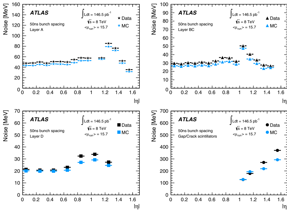
Fig. 11 The total noise per cell as a function of |\eta| for \langle \mu_{run} \rangle = 15.7 , for the high–high gain combination. The data from a 2012 run, with a bunch spacing of 50 ns, are shown in black while the simulation is
