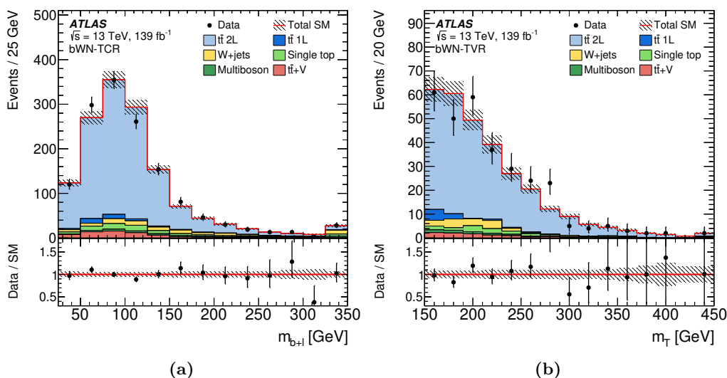
Figure 7. Selected distributions in the \mathbf{bWN} CR and VR: (a) m_{b+l} in the TCR, (b) m_T in the TVR. The distributions shown are post-fit, i.e. each background is scaled by a normalisation factor obtained from a background-only likelihood fit to the CRs (see table 14). The hatched area around the total SM prediction and the hatched band in the Data/SM ratio include all statistical and systematic uncertainties. The last (first) bin contains overflows (underflows).
