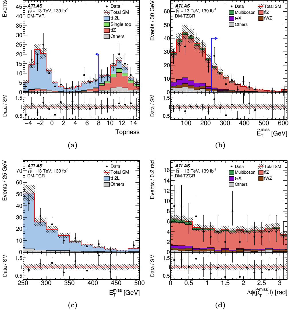
Figure 5. Selected kinematic distributions in DM CRs and VRs: (a) topness in the TVR before applying the topness selection, (b) \vec{E}_T^{\text{miss}} in the TZCR before applying the \vec{E}_T^{\text{miss}} selection, (c) E_T^{\text{miss}} in the TCR, (d) \Delta\phi(\vec{p}_T^{\text{miss}}, \ell) in the TZCR. For distributions where the requirement on the displayed variable is removed an arrow indicates the final selection on that variable. The distributions shown are post-fit, i.e. each background is scaled by a normalisation factor obtained from a background-only likelihood fit to the CRs (see table 14). The hatched area around the total SM prediction and the hatched band in the Data/SM ratio include all statistical and systematic uncertainties. The last (first) bin contains overflows (underflows).
