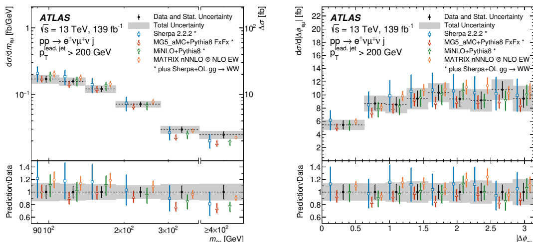
Figure 9. Measured fiducial cross-sections of WW +jets production for m_{e\mu} (left) and \Delta\phi(e,\mu) (right) in the fiducial phase space requiring p_T^{\text{lead, jet}} > 200 GeV. The last bin of the m_{e\mu} distribution is inclusive and the corresponding integrated cross-section is indicated by the right-hand-side axis. The measured cross-section values are shown as points with error bars giving the statistical uncertainty and solid bands indicating the size of the total uncertainty. The results are compared with the NNLO prediction with extra NLO EW corrections and NLO corrections for gg \rightarrow WW production (denoted MATRIX \otimes NLO EW) as well as NLO+PS predictions from SHERPA 2.2.2, MADGRAPH5_aMC@NLO + PYTHIA 8 with FxFx merging, and POWHEG MINLO + PYTHIA 8 for q\bar{q} initial states, combined with SHERPA + OPENLOOPS (LO+PS) for the gg initial state. The SHERPA 2.2.2 + OPENLOOPS prediction is normalized to the total cross-section calculated at NLO in QCD. Theoretical predictions are indicated as markers with vertical lines denoting PDF and scale uncertainties.
