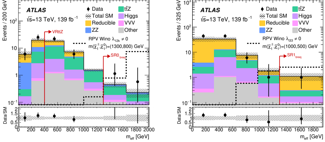
(a) m_{\text{eff}} in \text{SR0}_{\text{breq}} .
