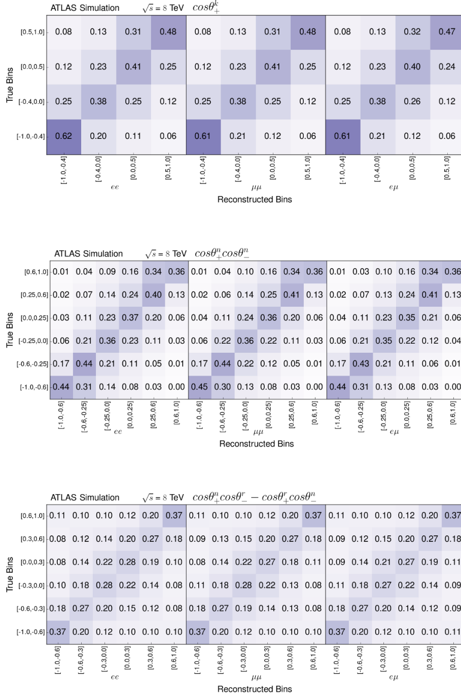
Figure 4. Response matrices of observables \cos\theta_+^k , \cos\theta_+^n \cos\theta_-^n , and \cos\theta_+^n \cos\theta_-^r - \cos\theta_+^r \cos\theta_-^n at parton level. They are divided into ee , \mu\mu , and e\mu channels. The matrices are normalised per truth bin (rows) for each channel separately.
