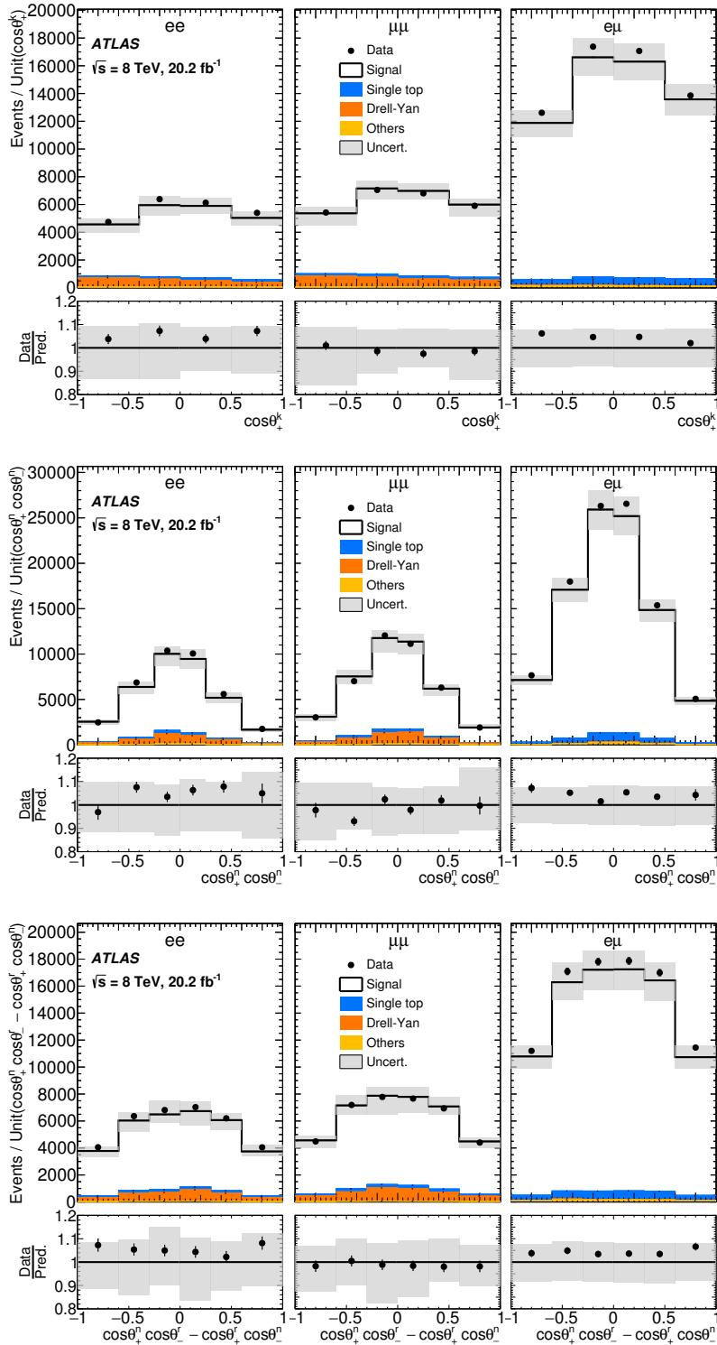
Figure 3. Input distributions for the unfolding procedure of \cos\theta_+^k , \cos\theta_+^n \cos\theta_-^n , and \cos\theta_+^n \cos\theta_-^r - \cos\theta_+^r \cos\theta_-^n . The ratio between the data and prediction is also shown. The grey area shows the total uncertainty on the signal and background. The t\bar{t}V , diboson and fake-lepton backgrounds are shown together in the “Others” category.
