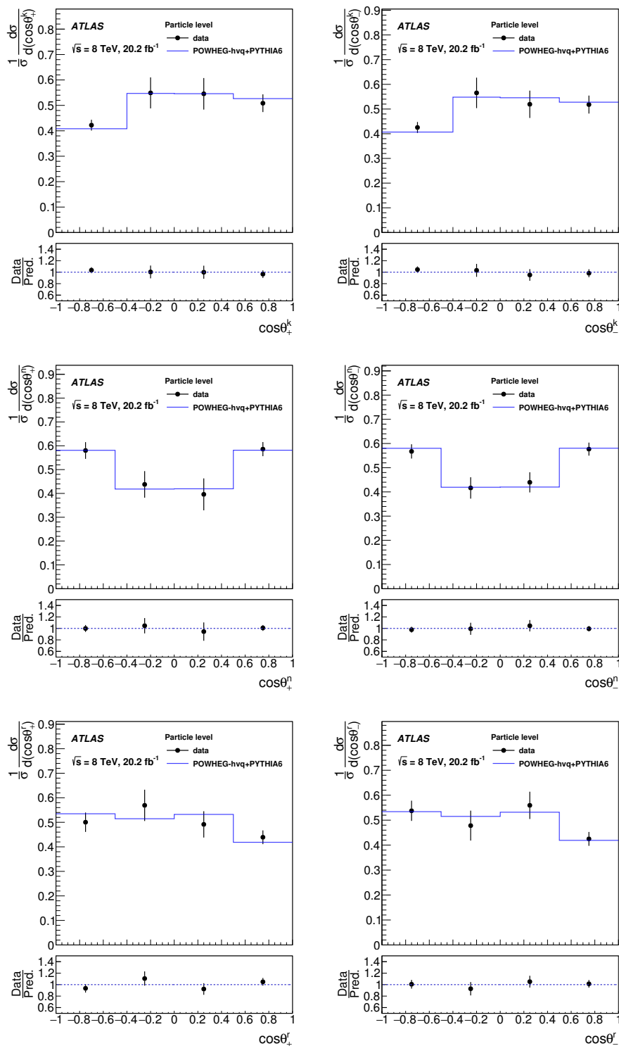
Figure 6. Comparison of the unfolded polarisation distributions and the prediction from the signal MC simulation for the stable-particle measurement. The total uncertainty is shown in each bin. The bin-to-bin correlations between adjacent bins are typically between -0.9 and -0.6 . The correlations between non-adjacent bins range from -0.4 to 0.6 .
