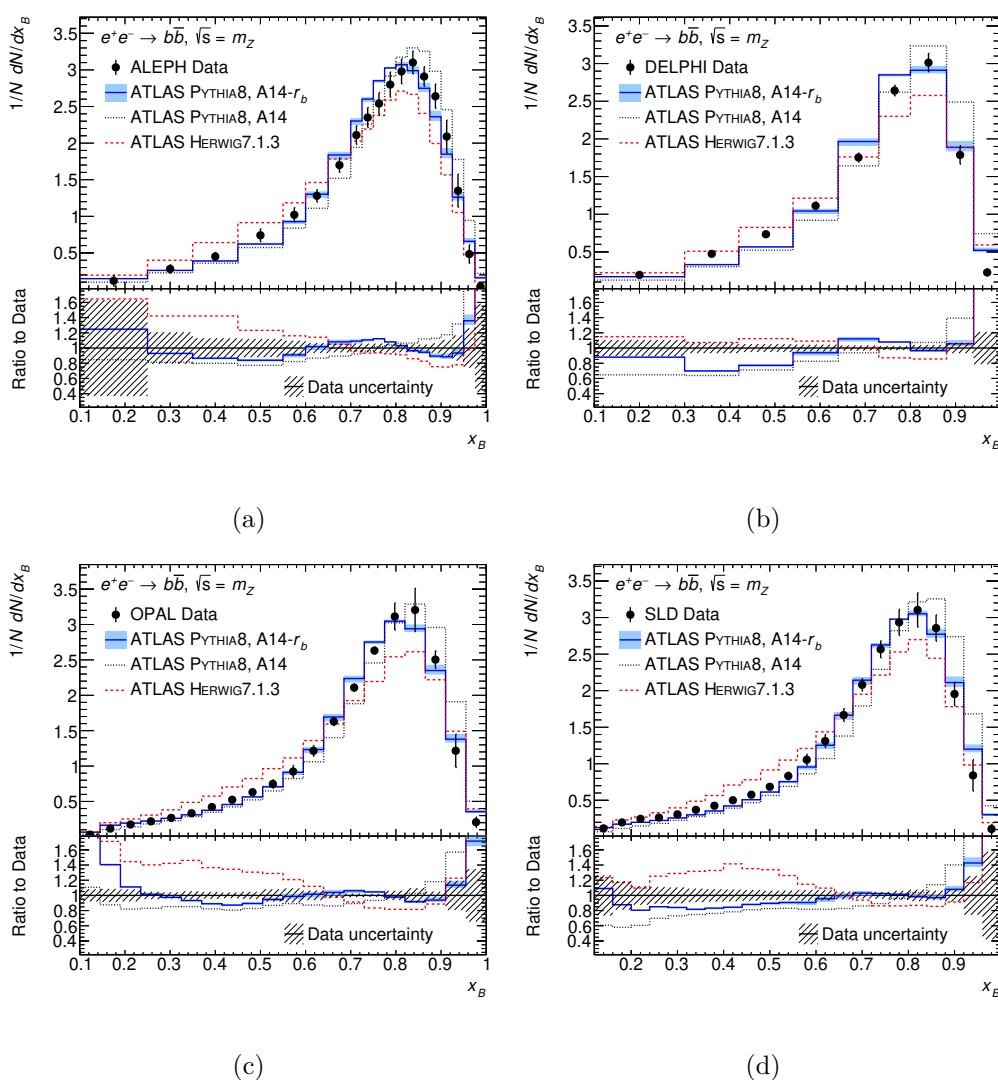
Figure 2. Distributions of x_B from semileptonically decaying b -hadrons in e^+e^- \rightarrow Z \rightarrow b\bar{b} events as measured by the ALEPH, DELPHI and OPAL experiments at the LEP collider, and by the SLD experiment at the SLC collider. Each of the measured spectra is compared with a set of MC predictions. The PYTHIA8 A14- r_b prediction includes a systematic uncertainty band obtained considering the r_b parameter variations described in the text and included as systematic uncertainty in the analysis.
