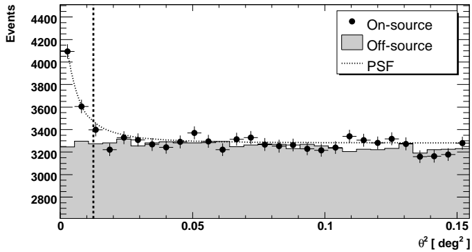
Fig. 1. Distribution of \theta^2 for on-source events (points) and normalized off-source events (shaded) from observations of H 2356–309. The dashed curve represents the expected distribution for a VHE \gamma -ray point source with photon index \Gamma = 3.06 at a zenith angle of 20^\circ . The vertical line denotes the on-source integration region relative to the nominal source position (Falomo 1991).
