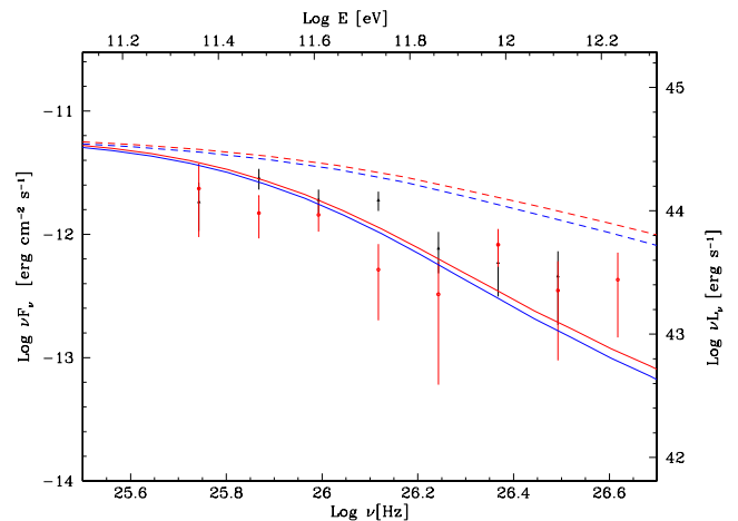
Fig. 9. SED of H 2356-309 zoomed in on the VHE band. The data and model curves are identical to those in Figure 8.
