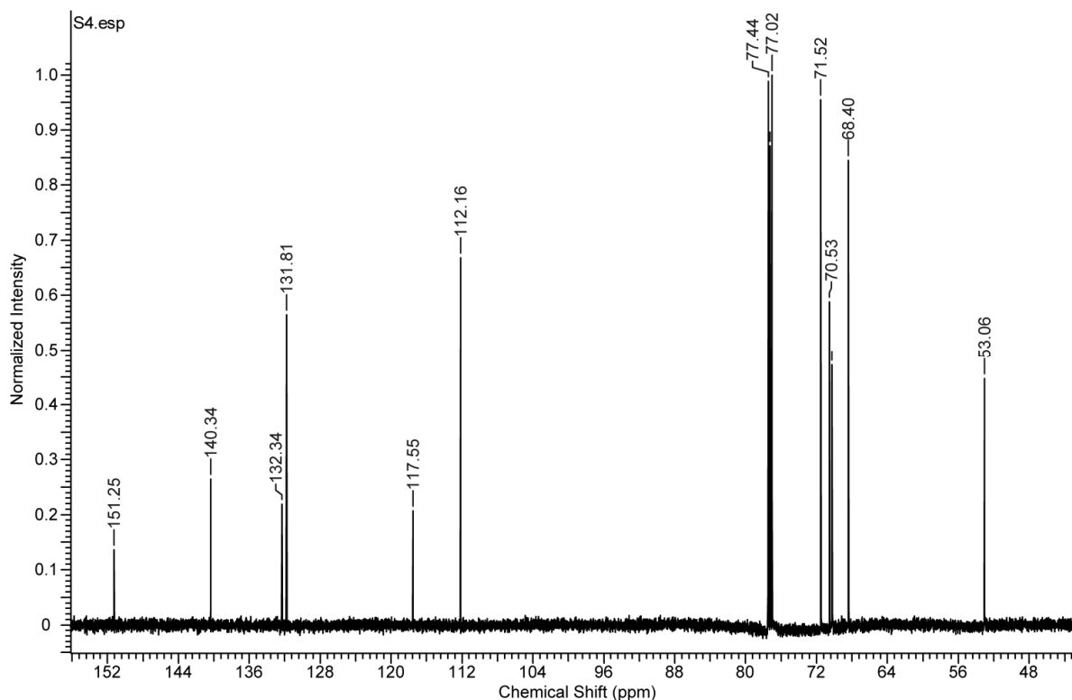
Figure S6. 600 MHz ^1\text{H} NMR spectrum of 4-aminoethyl-phenylaza-15-crown-5 ( 7 ).
