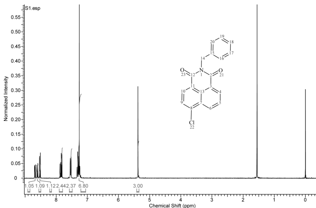
Figure S2. 300 MHz ^1\text{H} NMR spectrum of N -benzyl-4-chloro-1,8-naphthalimide ( 3 ) in \text{CDCl}_3 .
