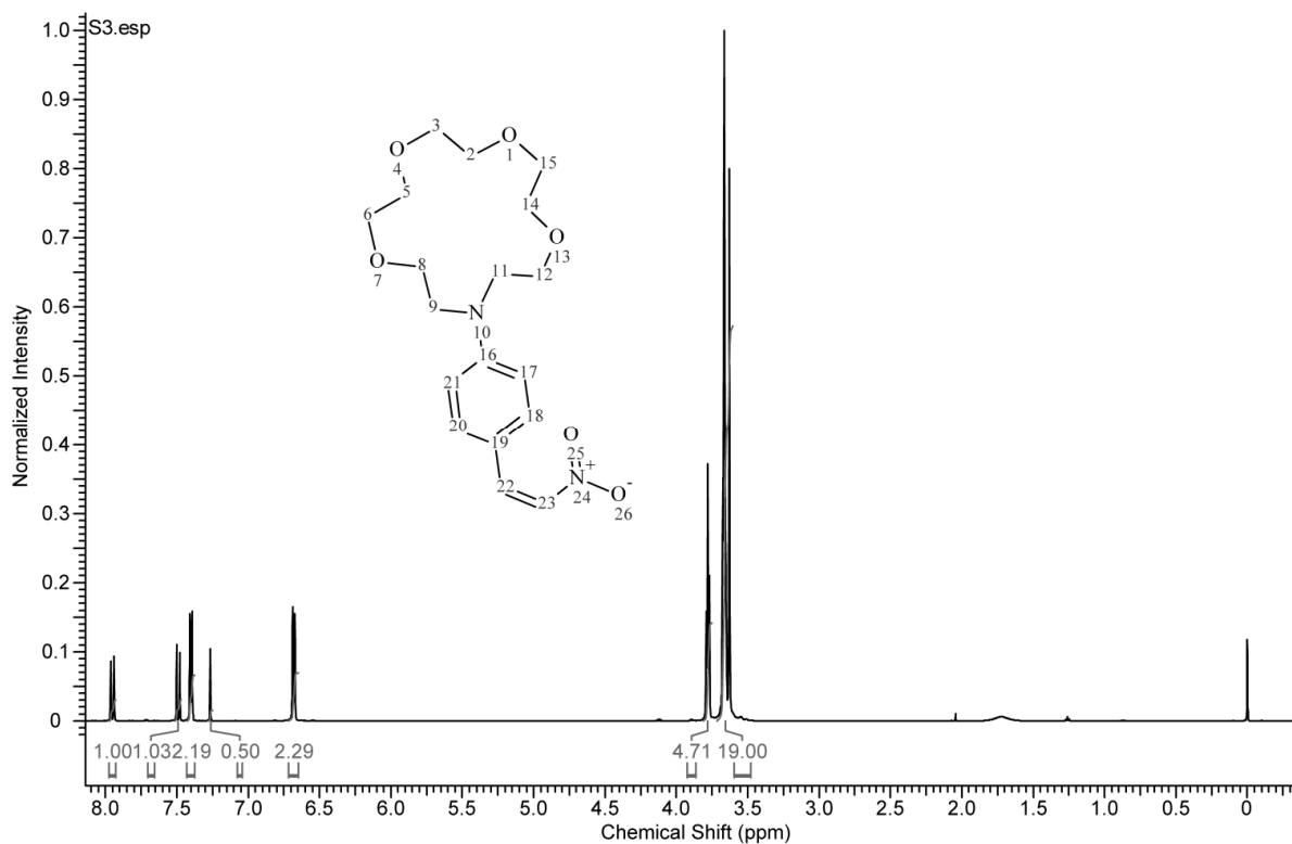
Figure S4. 600 MHz ^1\text{H} NMR spectrum of 4-nitroethenyl-phenylaza-15-crown-5 ( 6 ).
