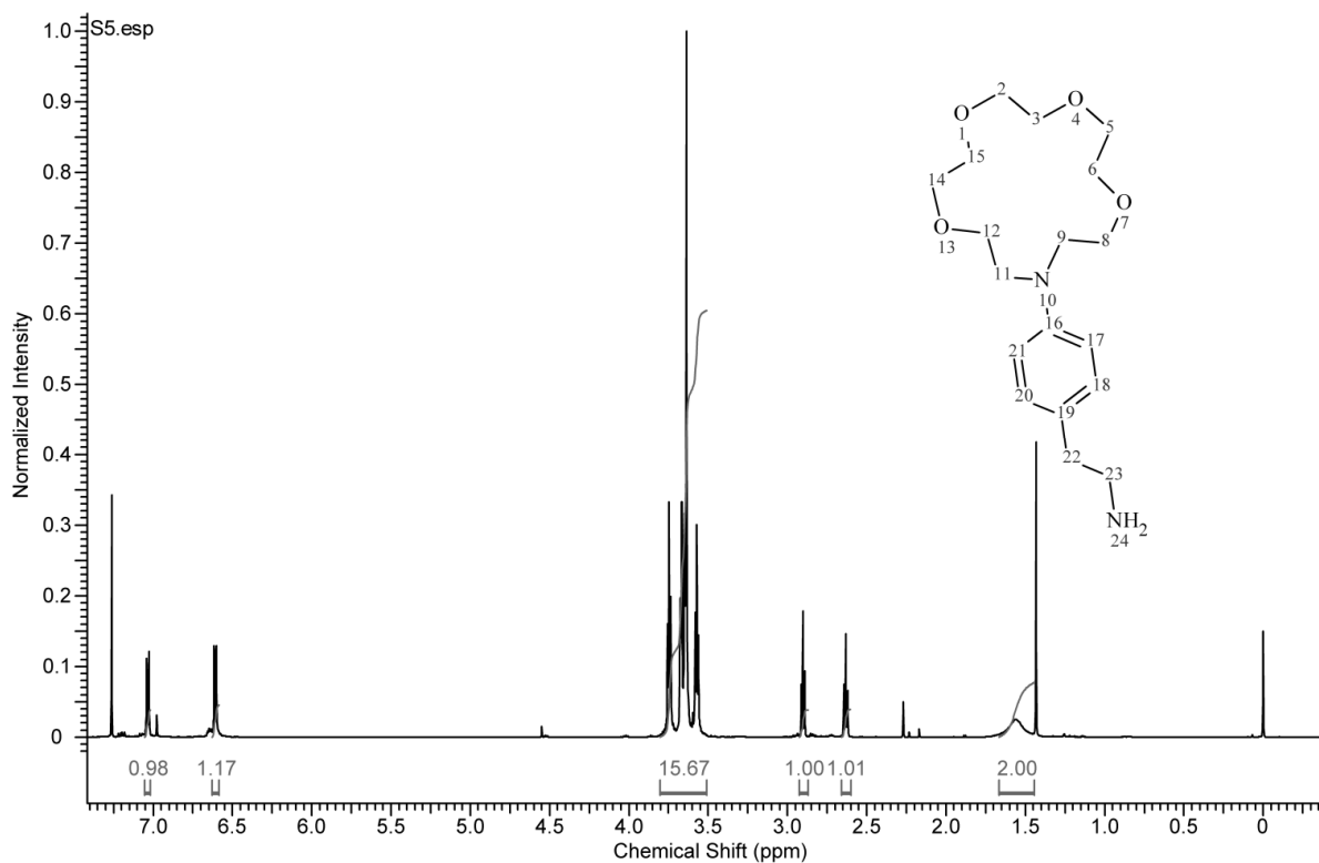
Figure S6. 600 MHz ^1\text{H} NMR spectrum of 4-aminoethyl-phenylaza-15-crown-5 ( 7 ).
