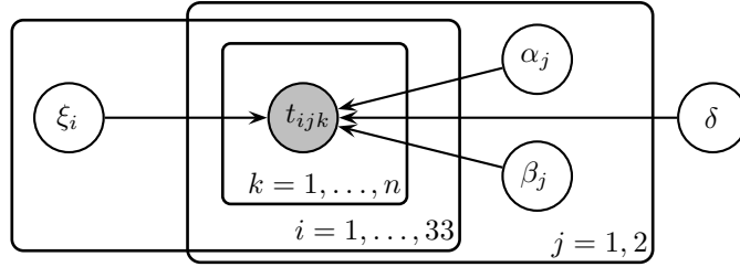
Figure 3: Graphical model for the benchmark data analysis.
